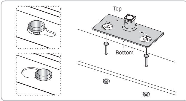
Short Bolt (2EA)
